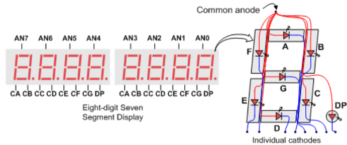
( https://digilent.com/reference/_detail/reference/programmable-logic/nexys-a7/n4u.png?id=programmable-logic%3Anexys-a7%3Areference-manual ) Figure 9.1.2 Common Anode Circuit Node
