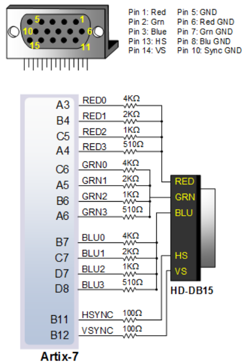
( https://digilent.com/reference/_detail/reference/programmable-logic/nexys-a7/n4m.png?id=programmable-logic%3Anexys-a7%3Areference-manual ) Figure 8.1 Nexys A7 VGA Interface
