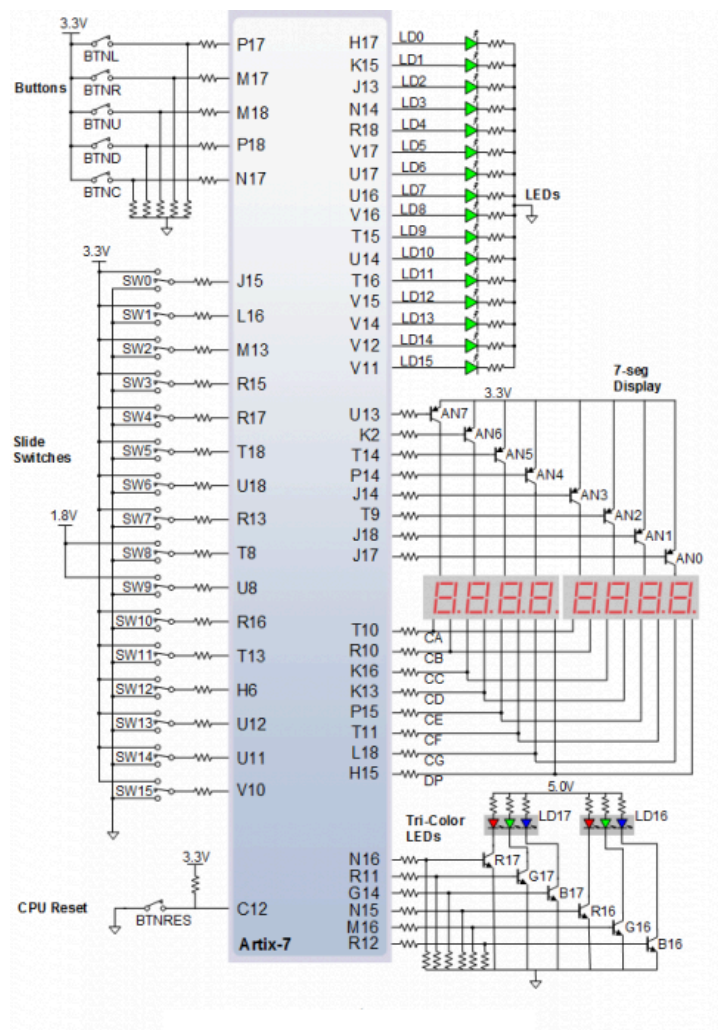
( https://digilent.com/reference/_detail/reference/programmable-logic/nexys-a7/n4s.png?id=programmable-logic%3Anexys-a7%3Areference-manual ) Figure 9.1 General Purpose I/O Devices on the Nexys A7
