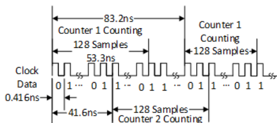
( https://digilent.com/reference/_detail/reference/programmable-logic/nexys-a7/n4ad.png?id=programmable-logic%3Anexys-a7%3Areference-manual ) Figure 14.2.2 Sampling PDM with Two Counters
