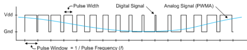
( https://digilent.com/reference/_detail/reference/programmable-logic/nexys-a7/n4ag.png?id=programmable-logic%3Anexys-a7%3Areference-manual ) Figure 15.1.1 Simple Waveform Represented as PWM
