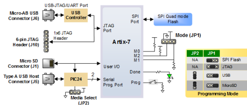
( https://digilent.com/reference/_detail/reference/programmable-logic/nexys-a7/n4e.png?id=programmable-logic%3Anexys-a7%3Areference-manual ) Figure 2.1 Nexys A7 Configuration Options
