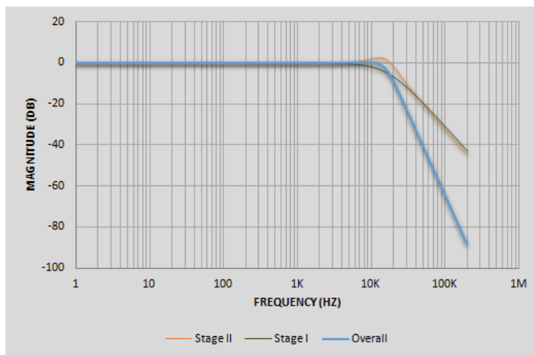
( https://digilent.com/reference/_detail/reference/programmable-logic/nexys-a7/n4af.png?id=programmable-logic%3Anexys-a7%3Areference-manual ) Figure 15.2 SK Butterworth Low-Pass Filter Frequency Response
