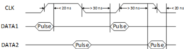
( https://digilent.com/reference/_detail/reference/programmable-logic/nexys-a7/n4ac.png?id=programmable-logic%3Anexys-a7%3Areference-manual ) Figure 14.2.1 PDM Timing Diagram
