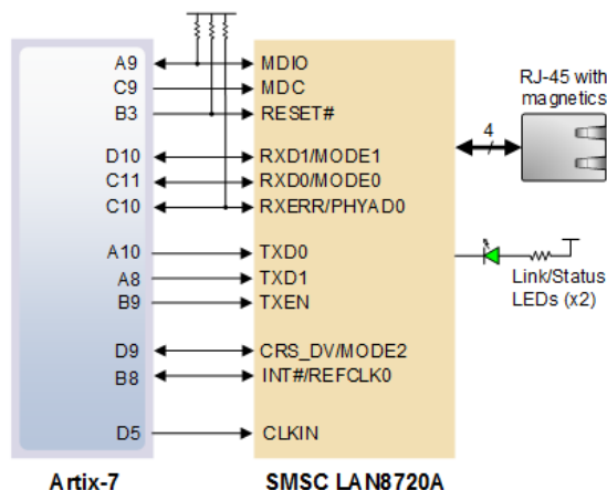
( https://digilent.com/reference/_detail/reference/programmable-logic/nexys-a7/n4g.png?id=programmable-logic%3Anexys-a7%3Areference-manual ) Figure 4.1 Pin Connections between the AMD Artix™ 7 and the Ethernet PHY
