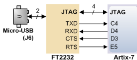
( https://digilent.com/reference/_detail/reference/programmable-logic/nexys-a7/n4g.png?id=programmable-logic%3Anexys-a7%3Areference-manual ) Figure 6.1 Nexys A7 FT2232HQ Connections
