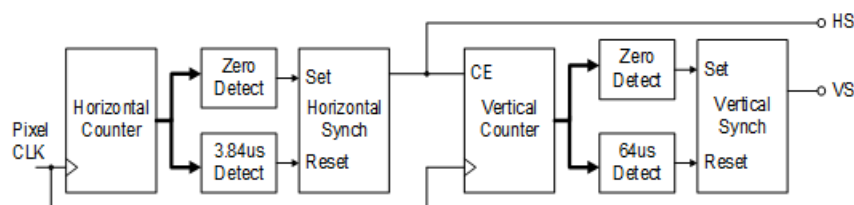
( https://digilent.com/reference/_detail/reference/programmable-logic/nexys-a7/n4q.png?id=programmable-logic%3Anexys-a7%3Areference-manual ) Figure 8.1.4 VGA Display Controller Block Diagram
