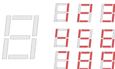
( https://digilent.com/reference/_detail/reference/programmable-logic/nexys-a7/n4s.png?id=programmable-logic%3Anexys-a7%3Areference-manual ) Figure 9.1.1 An Un-illuminated Seven-Segment Display and Nine Illumination Patterns Corresponding to Decimal Digits
