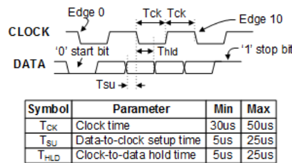
( https://digilent.com/reference/_detail/reference/programmable-logic/nexys-a7/n4i.png?id=programmable-logic%3Anexys-a7%3Areference-manual ) Figure 7.1.1 PS/2 Device-to-Host Timing Diagram
