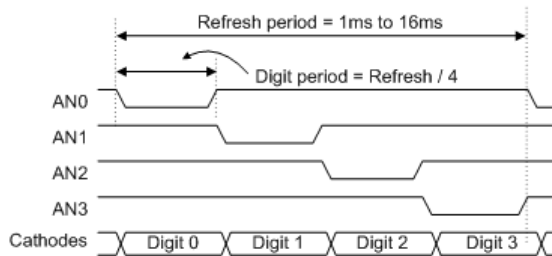
( https://digilent.com/reference/_detail/reference/programmable-logic/nexys-a7/n4u.png?id=programmable-logic%3Anexys-a7%3Areference-manual ) Figure 9.1.3 Four Digit Scanning Display Controller Timing Diagram
