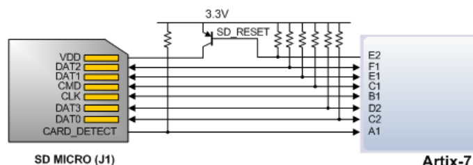
( https://digilent.com/reference/_detail/reference/programmable-logic/nexys-a7/n4w.png?id=programmable-logic%3Anexys-a7%3Areference-manual ) Figure 11.1 AMD Artix™ 7 microSD Card Connector Interface (PIC24 Connections not Shown)
