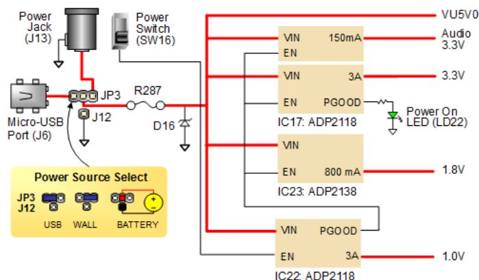
( https://digilent.com/reference/_detail/reference/programmable-logic/nexys-a7/n4d.png?id=programmable-logic%3Anexys-a7%3Areference-manual ) Figure 1.1 Nexys A7 Power Circuit
