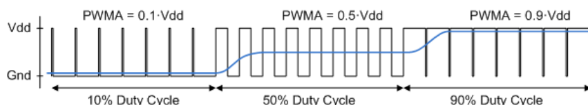
( https://digilent.com/reference/_detail/reference/programmable-logic/nexys-a7/n4ah.png?id=programmable-logic%3Anexys-a7%3Areference-manual ) Figure 15.1.2 Representation of a PWM Integrator Producing an Output Voltage by Integrating the Pulse Train
