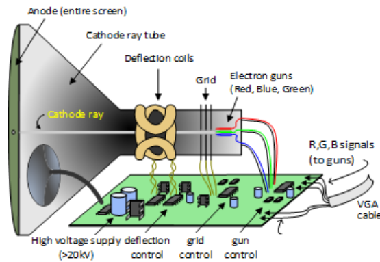
( https://digilent.com/reference/_detail/reference/programmable-logic/nexys-a7/n4n.png?id=programmable-logic%3Anexys-a7%3Areference-manual ) Figure 8.1.1 Color CRT Display
