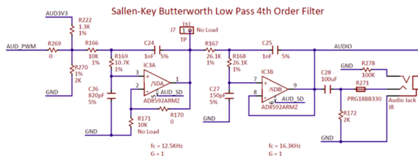
( https://digilent.com/reference/_detail/reference/programmable-logic/nexys-a7/n4ae.png?id=programmable-logic%3Anexys-a7%3Areference-manual ) Figure 15.1 Sallen-Key Butterworth Low-Pass 4th Order Filter
