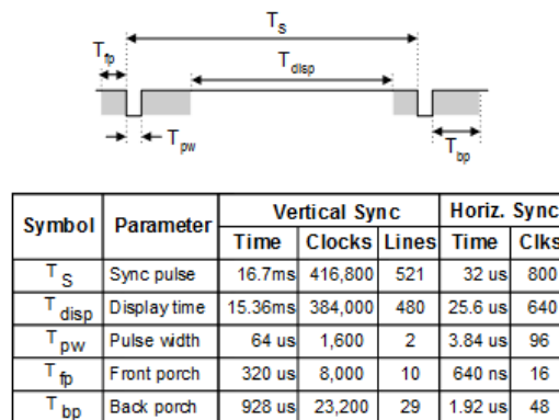
( https://digilent.com/reference/_detail/reference/programmable-logic/nexys-a7/n4p.png?id=programmable-logic%3Anexys-a7%3Areference-manual ) Figure 8.1.3 Signal Timings for a 640-Pixel by 480-Row Display Using a 25 MHz pixel Clock and 60 Hz Vertical Refresh
