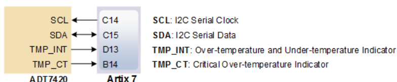
( https://digilent.com/reference/_detail/reference/programmable-logic/nexys-a7/n4x.png?id=programmable-logic%3Anexys-a7%3Areference-manual ) Figure 12.1 Temperature Sensor Interface
